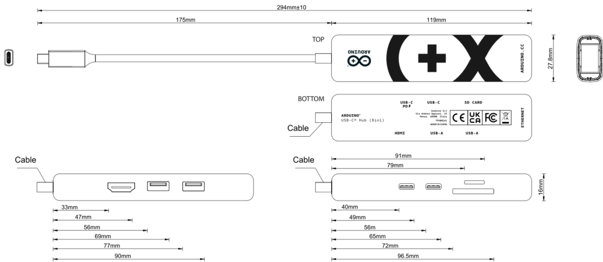
Hub Dimensions
