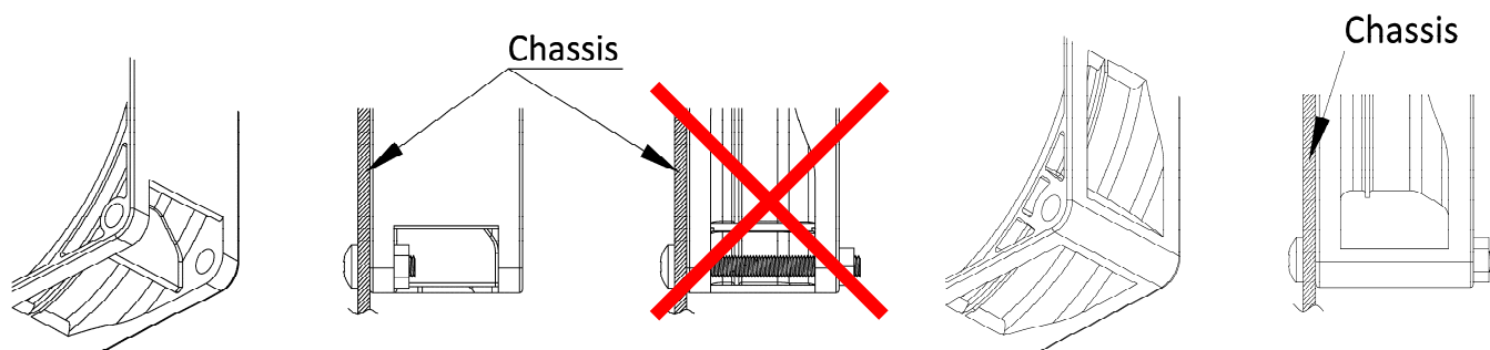
● FLANGE TYPE FIGURE 1
