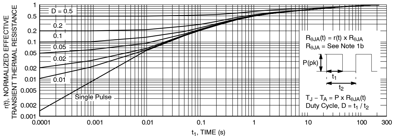
Figure 17. Transient Thermal Response Curve
