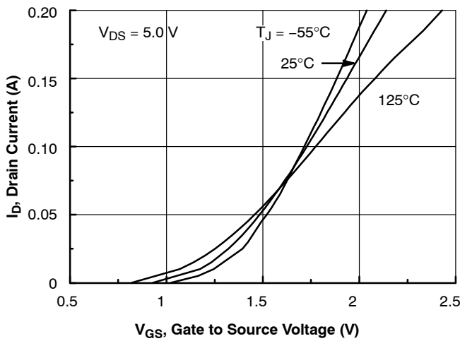
Figure 6. Transfer Characteristics
