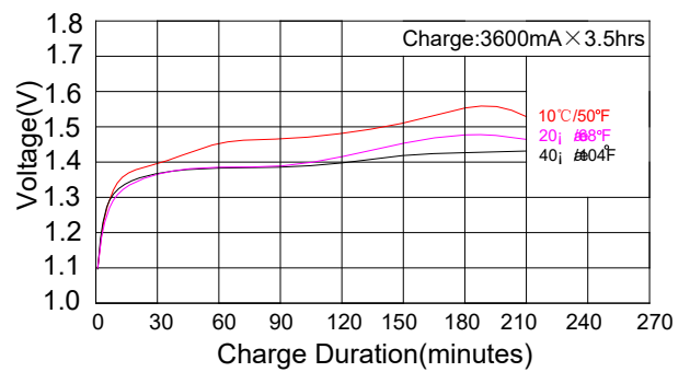
Fast charge characteristics
