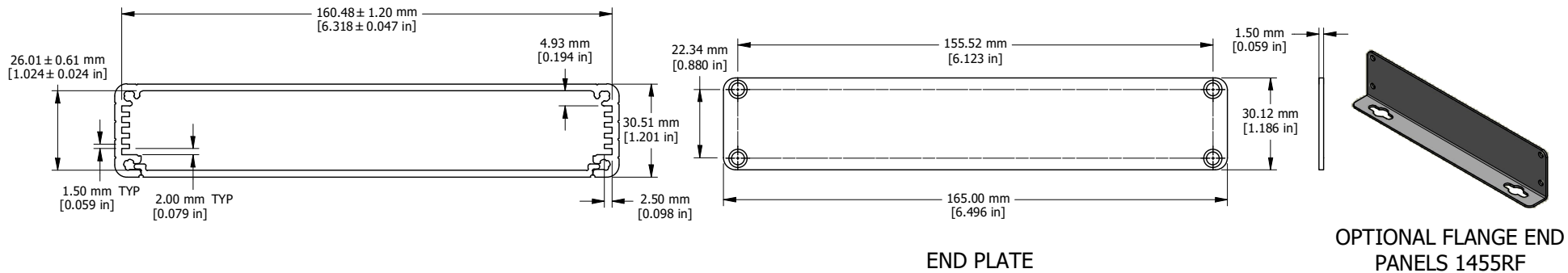
EXTRUSION
