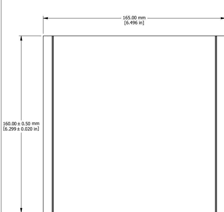
EXTRUSION
