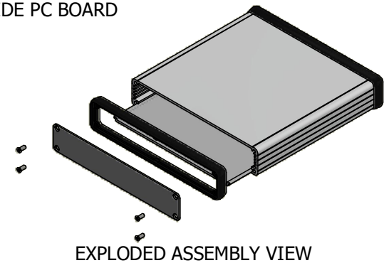
EXTRUSION DESIGNED FOR 160MM WIDE PC BOARD
