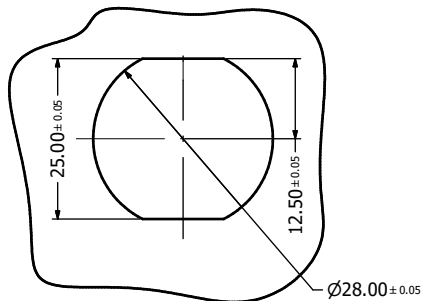
Recommended Double-D Panel Cutout
