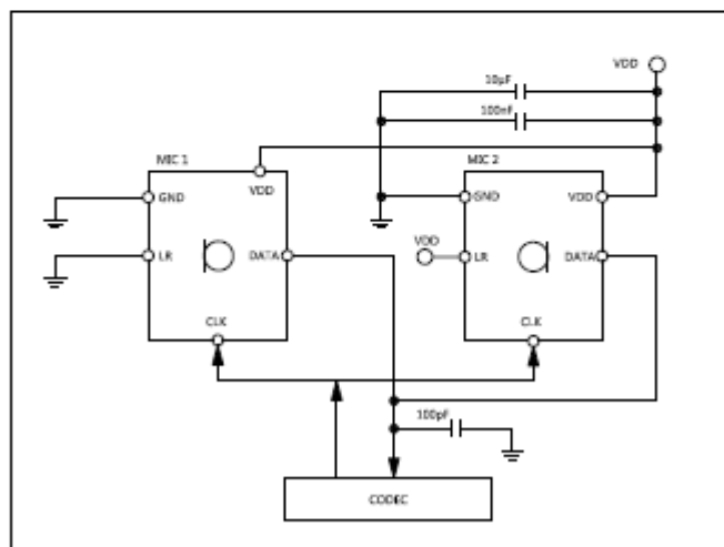
Figuer 2. Electrical connections for stereo configurations
