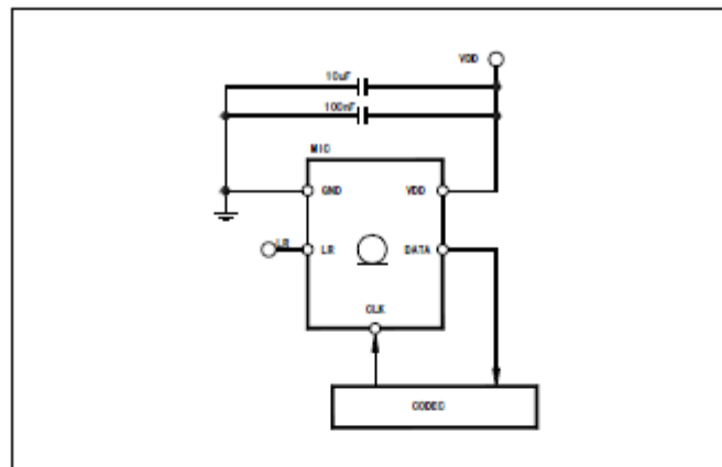
Figuer 2. Electrical connections for stereo configurations
