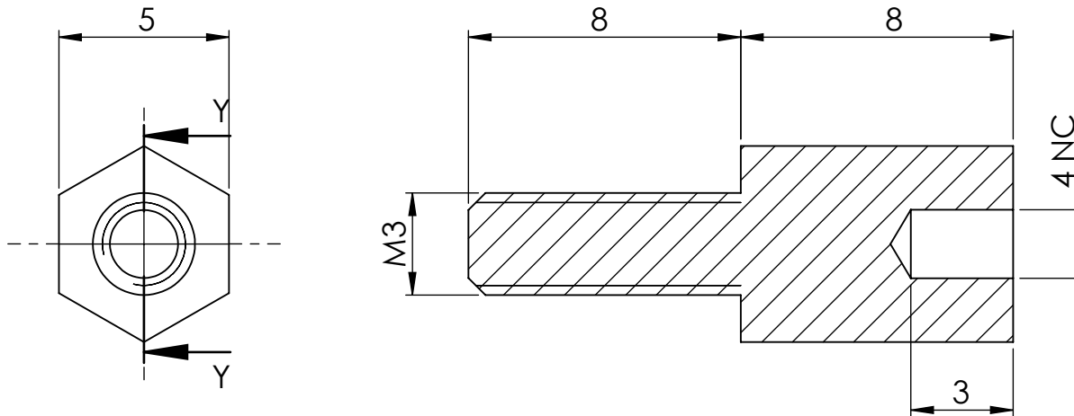
SECTION Y-Y
