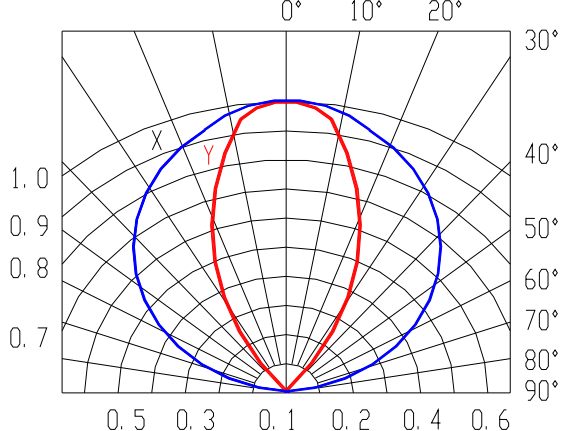
Radiation Characteristics
