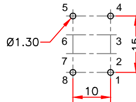
Viewed on component side
