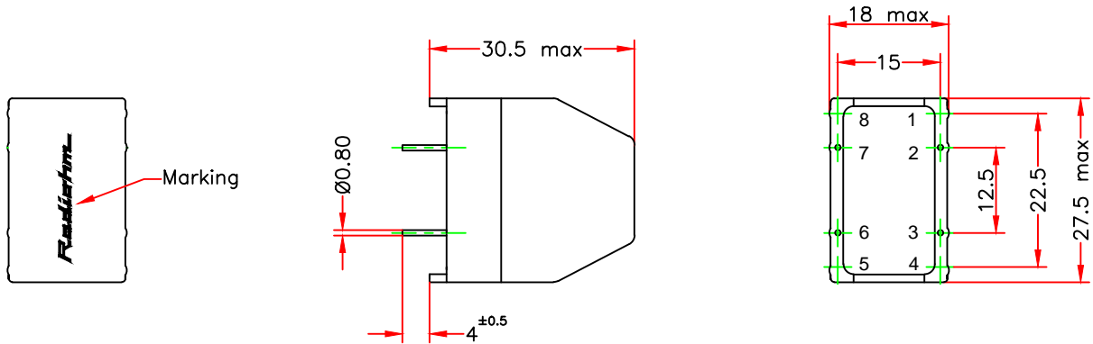
Viewed on component side
