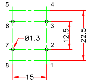
Viewed on component side
