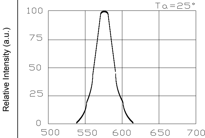
Relative Intensity vs. Wavelength ( T_a=25^\circ )
