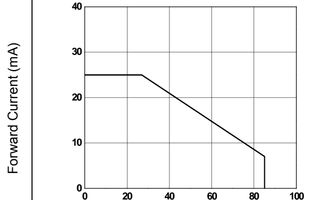
Forward Current vs. Ambient Temp.
