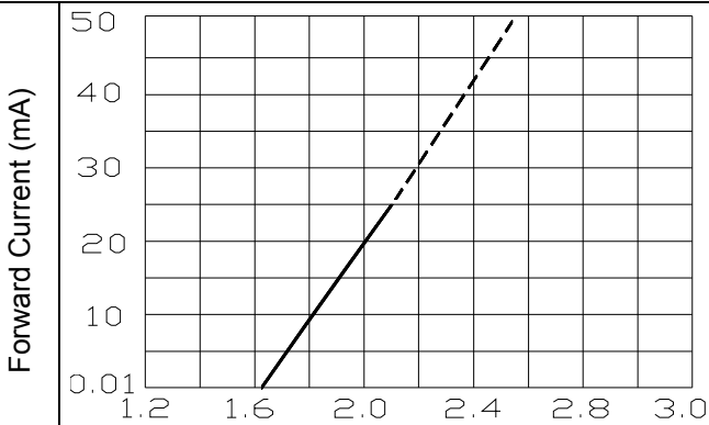
Forward Current vs. Forward Voltage ( T_a=25^\circ )
