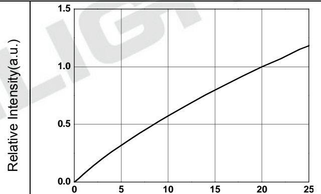
Relative Intensity vs. Forward Current ( T_a=25^\circ )
