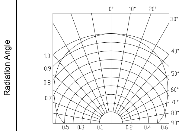
Directivity ( T_a=25^\circ )
