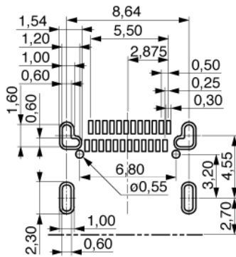
PCB layout
