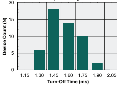
Typical Turn-Off Time (N=50, I_F=2mA , I_L=100mA )
