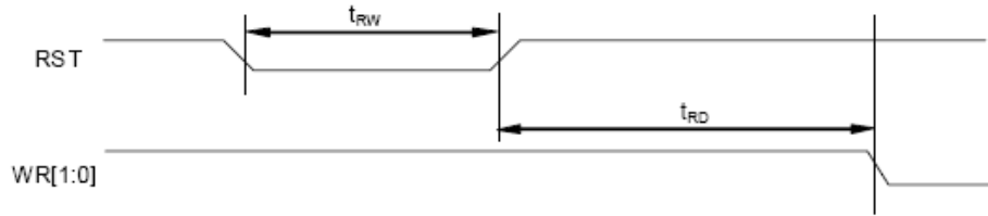
Reset Characteristics
