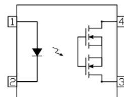
Pin Configuration
