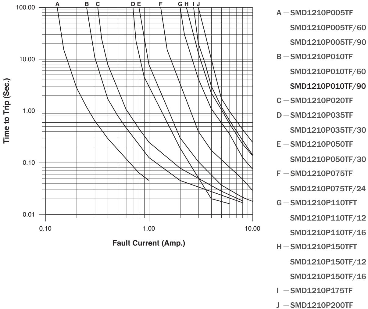
Average Time-Current Curve
