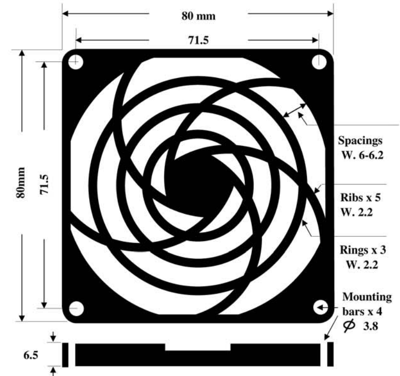
Guard "G" / G80P
