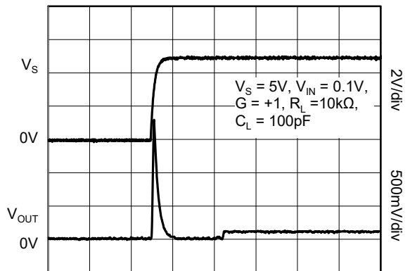
Time (20μs/div)
