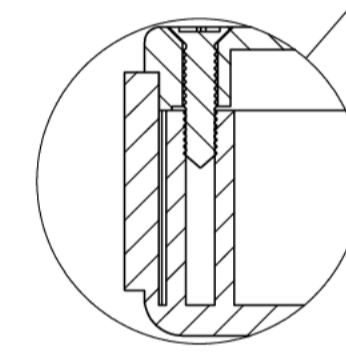
Detalle/Detail R Escala/Scale 2 : 1
