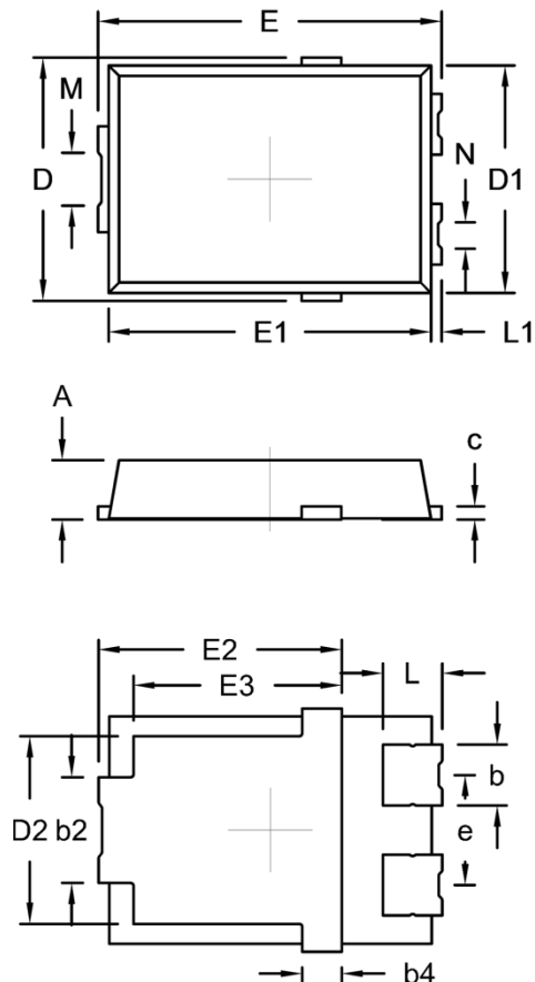
TO-277A (SMPC4.6U)
