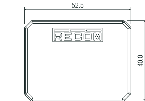
Dimension Drawing "/277" version SINGLE and DUAL Output (mm)
