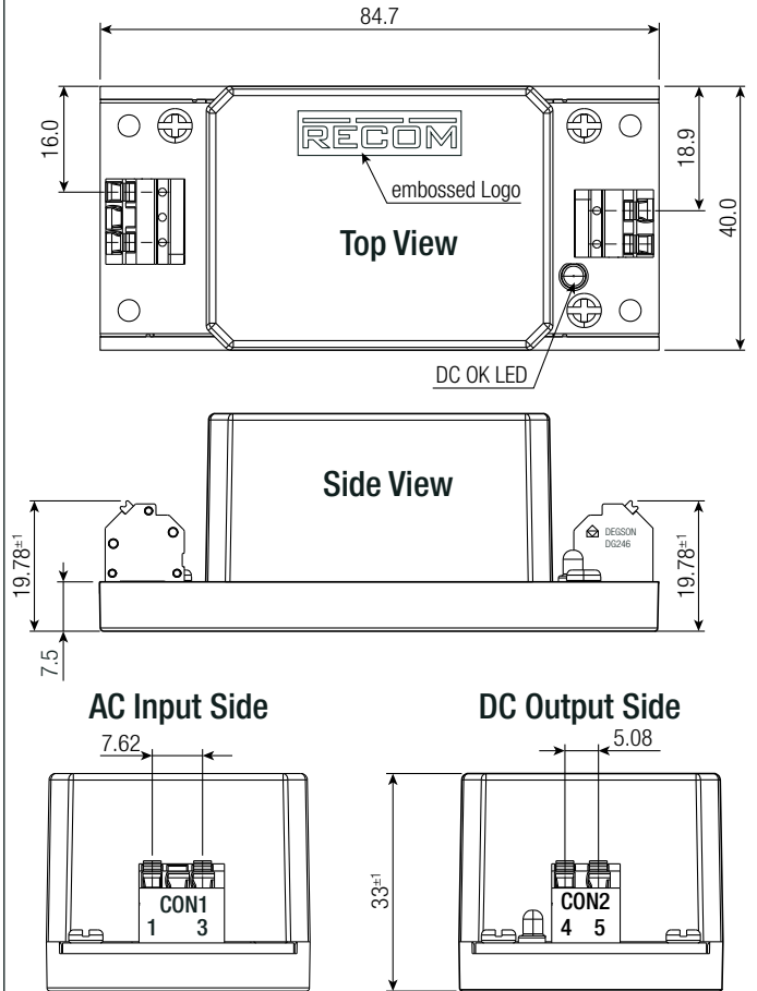
Dimension Drawing Panel Mount “/PMA” SINGLE Output (mm)
