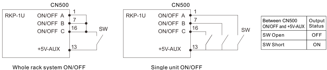
Figure 3-4 Connection for remote ON/OFF control operation
