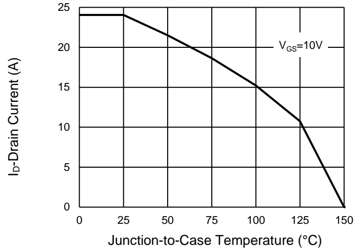
Drain Current
