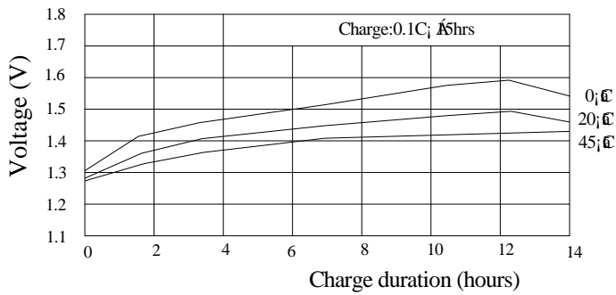
Standard charge characteristics
