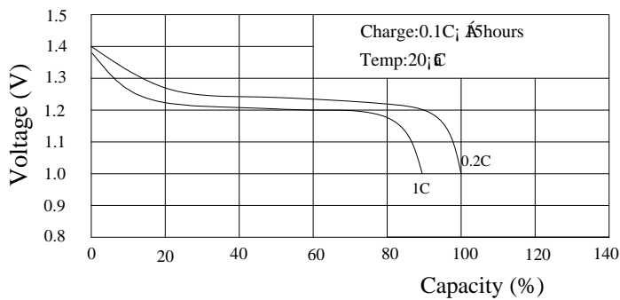
Discharge characteristics
