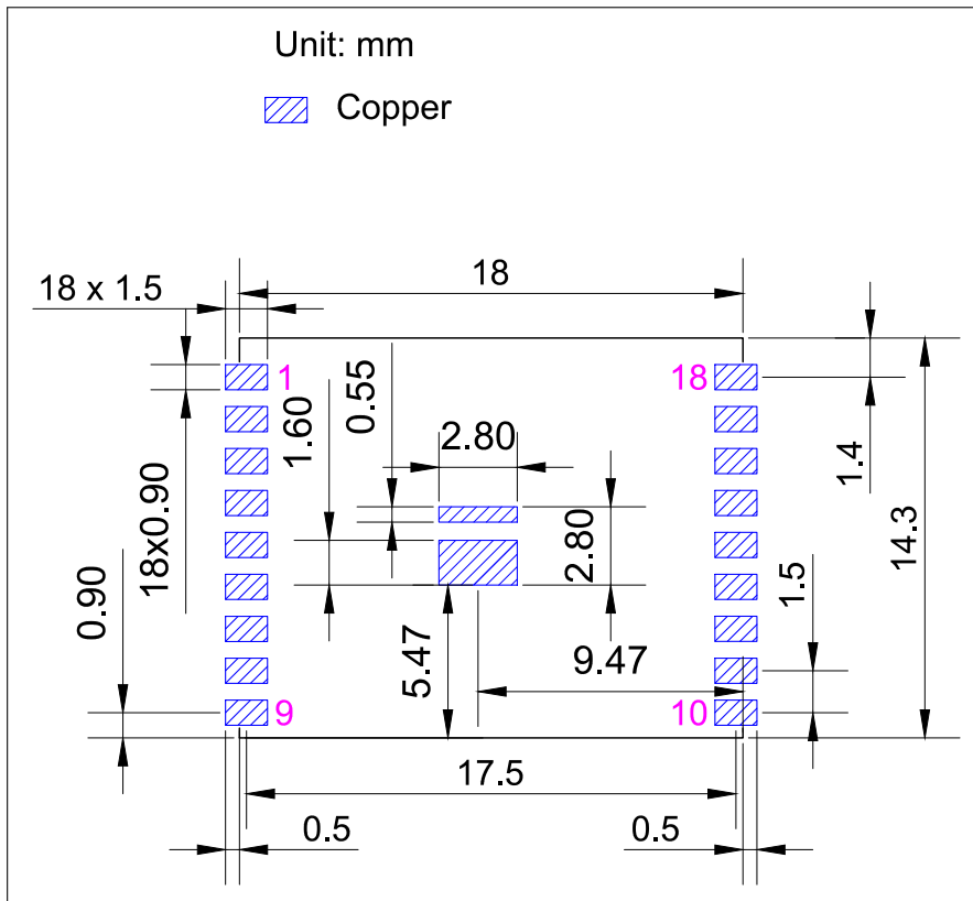
Figure 11: ESP8684-WROOM-02UC Recommended PCB Land Pattern
