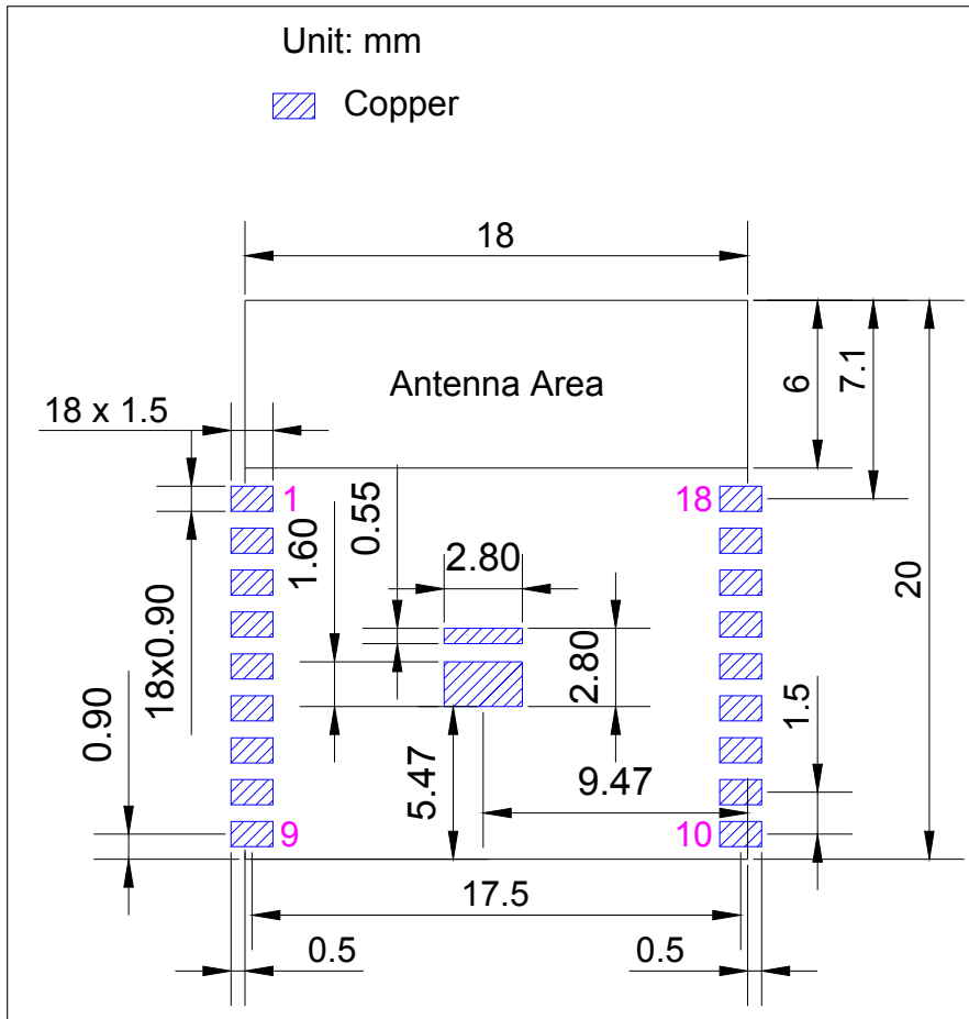
Figure 10: ESP8684-WROOM-02C Recommended PCB Land Pattern
