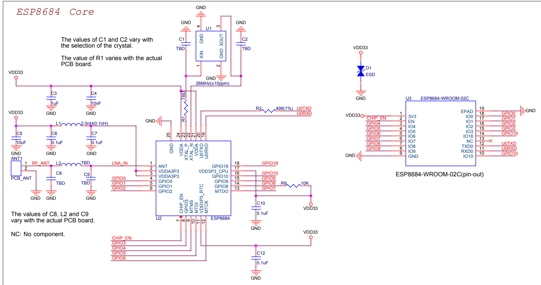
Figure 5: ESP8684-WROOM-02C Schematics
