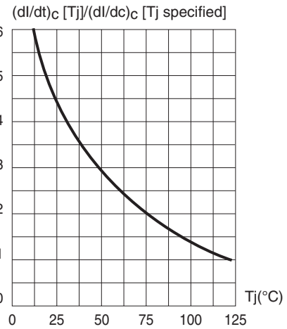
Fig. 8: Relative variation of critical rate of decrease of main current versus junction temperature
