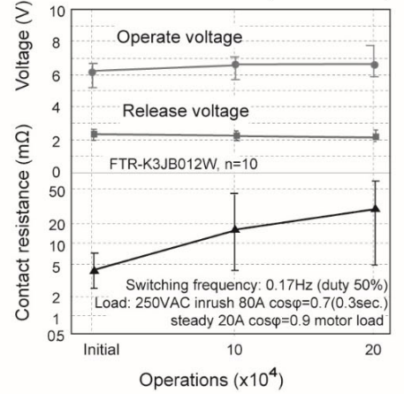
Electrical life test (motor load)
