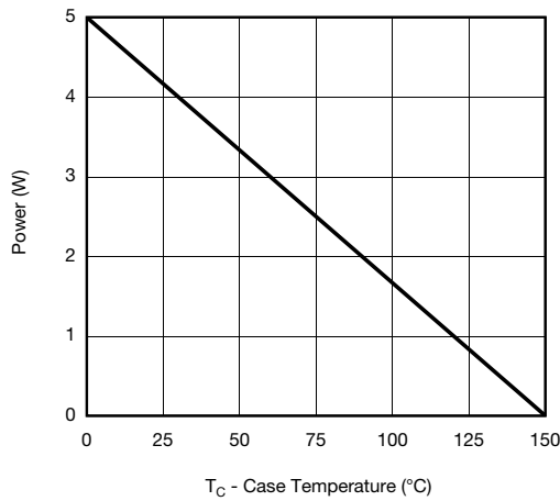
Power, Junction-to-Foot
