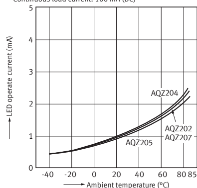
6-2. LED operate current vs. ambient temperature characteristics ( AC/DC type )
