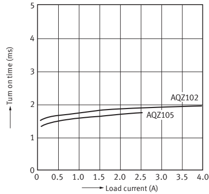
14-4. Turn on time vs. load current characteristics ( AC/DC type )
