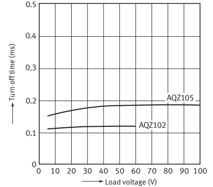
15-4. Turn off time vs. load voltage characteristics ( AC/DC type )
