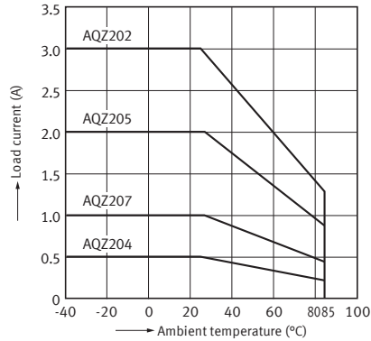
1-2. Load current vs. ambient temperature characteristics ( AC/DC type )
