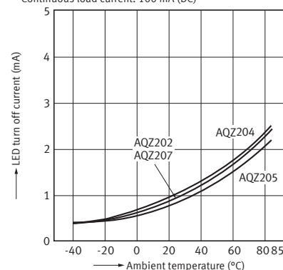
7-2. LED turn off current vs. ambient temperature characteristics ( AC/DC type )
