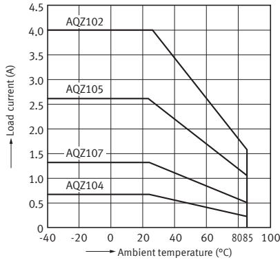
1-1. Load current vs. ambient temperature characteristics ( DC type )
