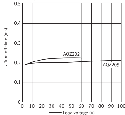
15-3. Turn off time vs. load voltage characteristics ( AC/DC type )
