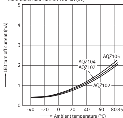
7-1. LED turn off current vs. ambient temperature characteristics ( DC type )
