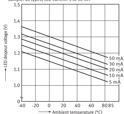
8. LED dropout voltage vs. ambient temperature characteristics
