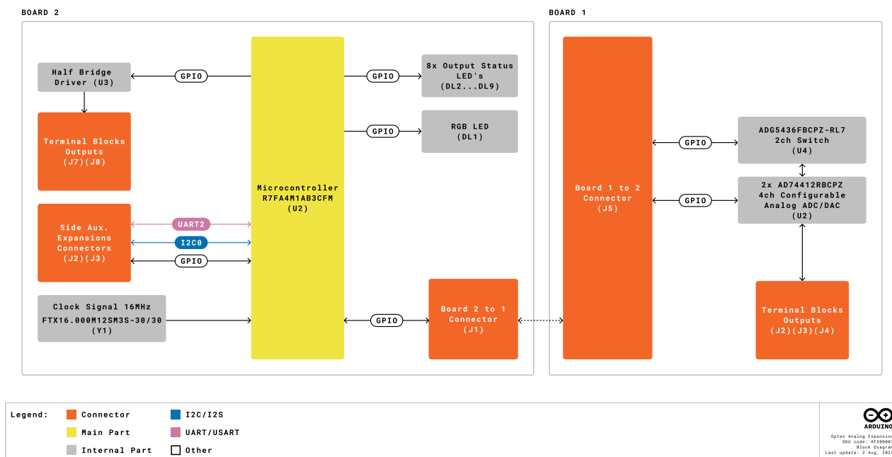
Block diagram
