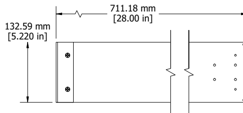
ASSEMBLY - SIDE VIEW
