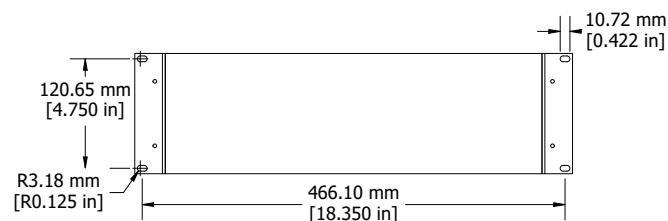
ASSEMBLY - FRONT VIEW
