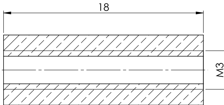
SECTION Y-Y
