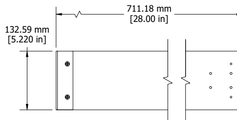
ASSEMBLY - SIDE VIEW
