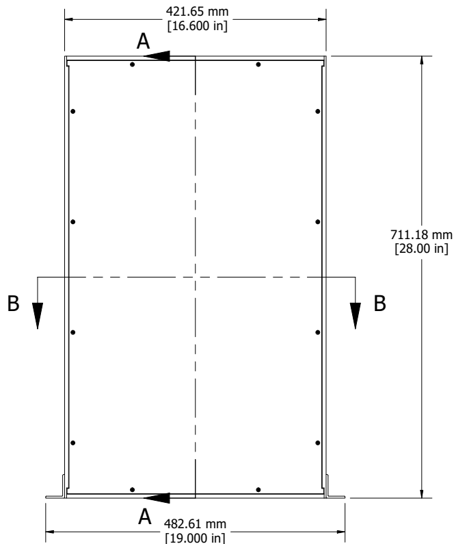
ASSEMBLY - TOP VIEW
