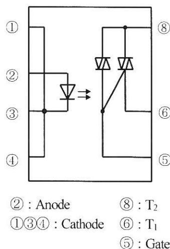
Pin-Number and internal connection diagram
