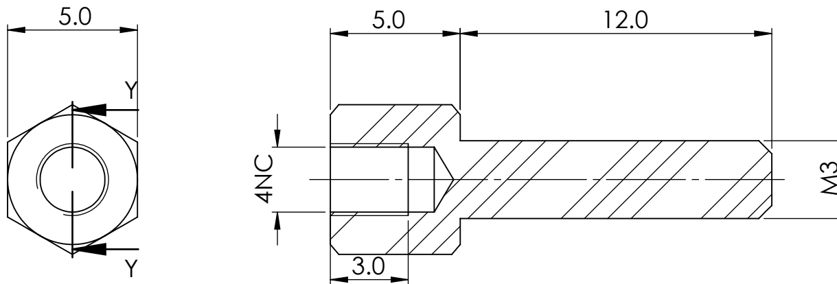
SECTION Y-Y
