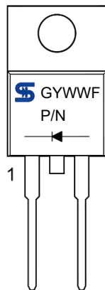
MARKING DIAGRAM
