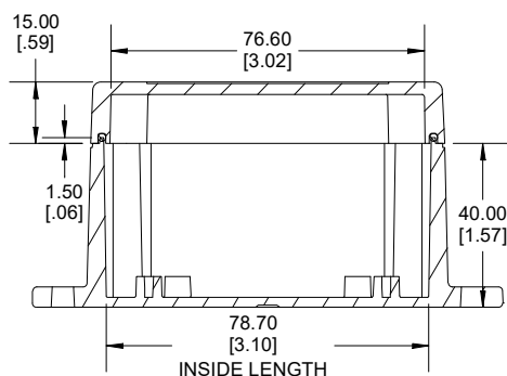
SIDE VIEW SECTION B-B
