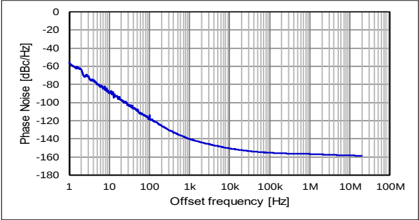
Phase Jitter (Offset frequency: 12 kHz to 20 MHz)
