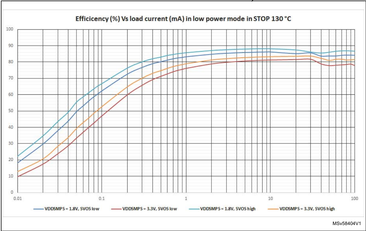
Figure 30. SMPS efficiency in SVOS mode T_J=130^{\circ}\text{C}
