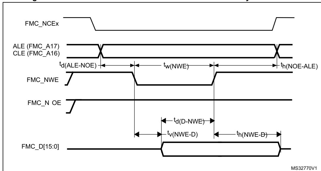
Figure 49. NAND controller waveforms for common memory write access
