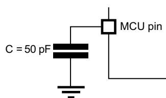
Figure 21. Pin loading conditions
