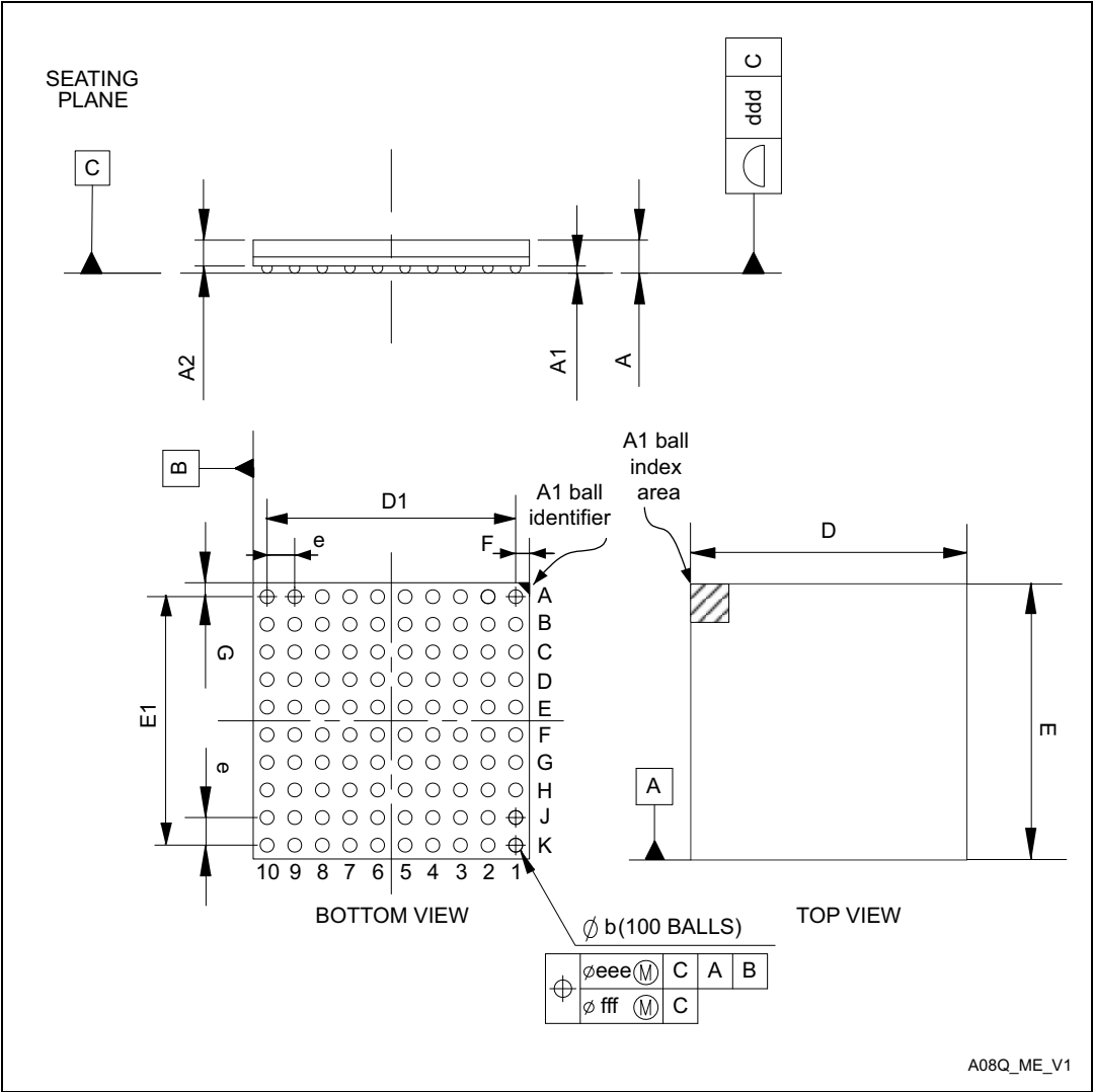
Figure 83. TFBGA100 - Outline
