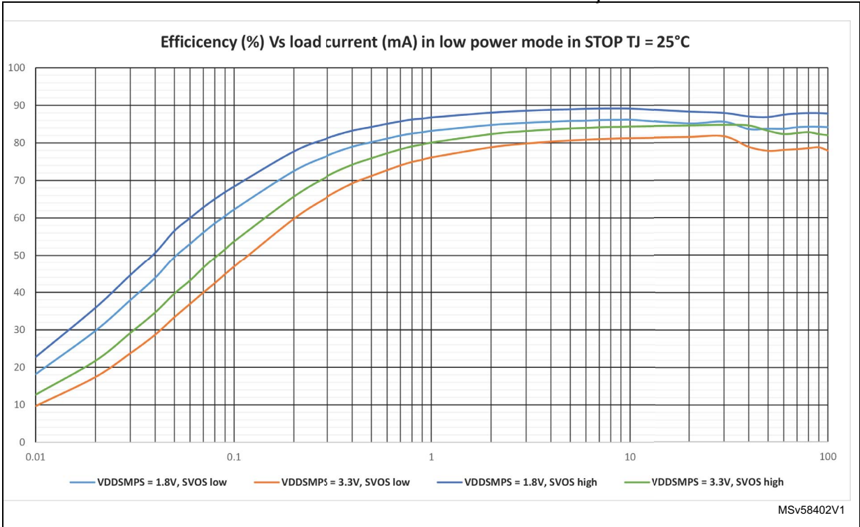
Figure 29. SMPS efficiency in SVOS mode T_J=25^{\circ}\text{C}
