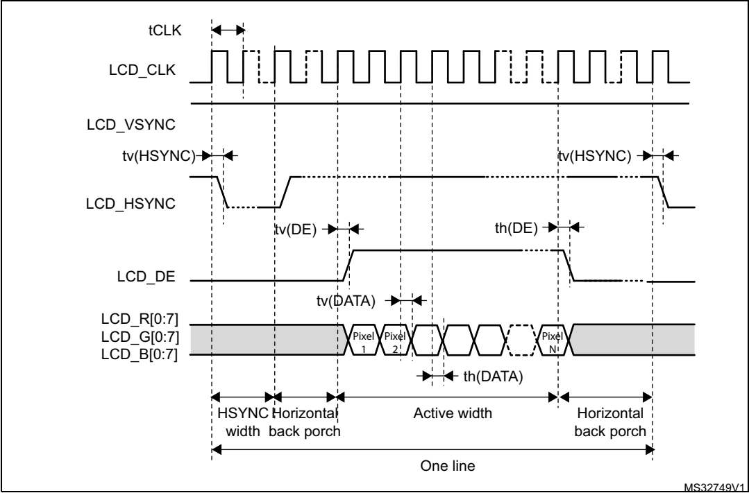
Figure 59. LCD-TFT horizontal timing diagram
