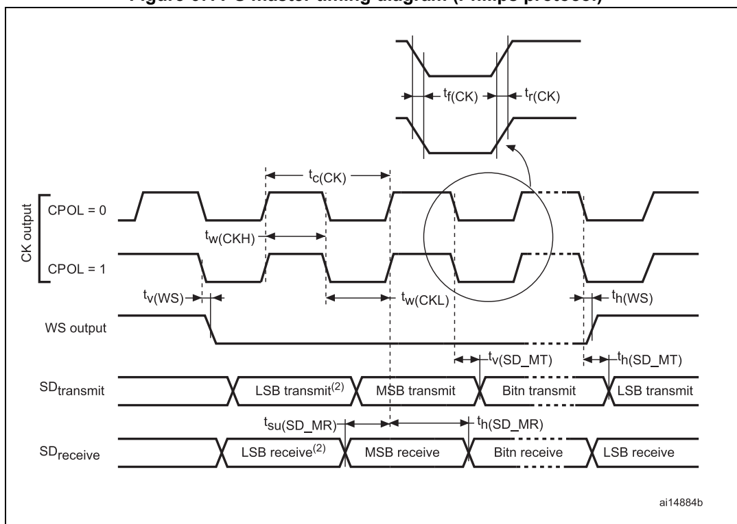
Figure 67. I 2 S master timing diagram (Philips protocol) (1)
