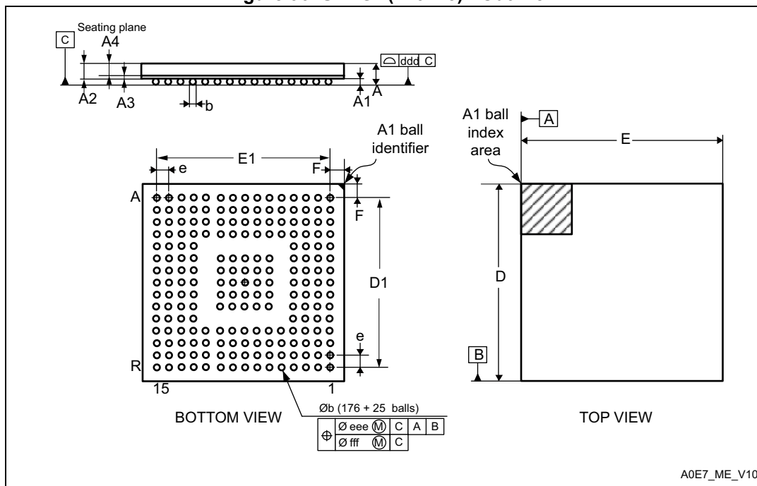
Figure 96. UFBGA(176+25) - Outline
