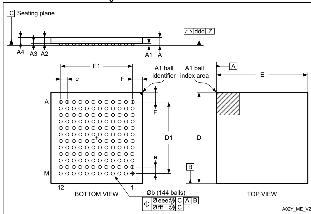
Figure 87. UFBGA144 - Outline
