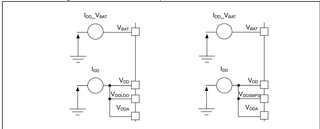
Figure 24. Current consumption measurement scheme
