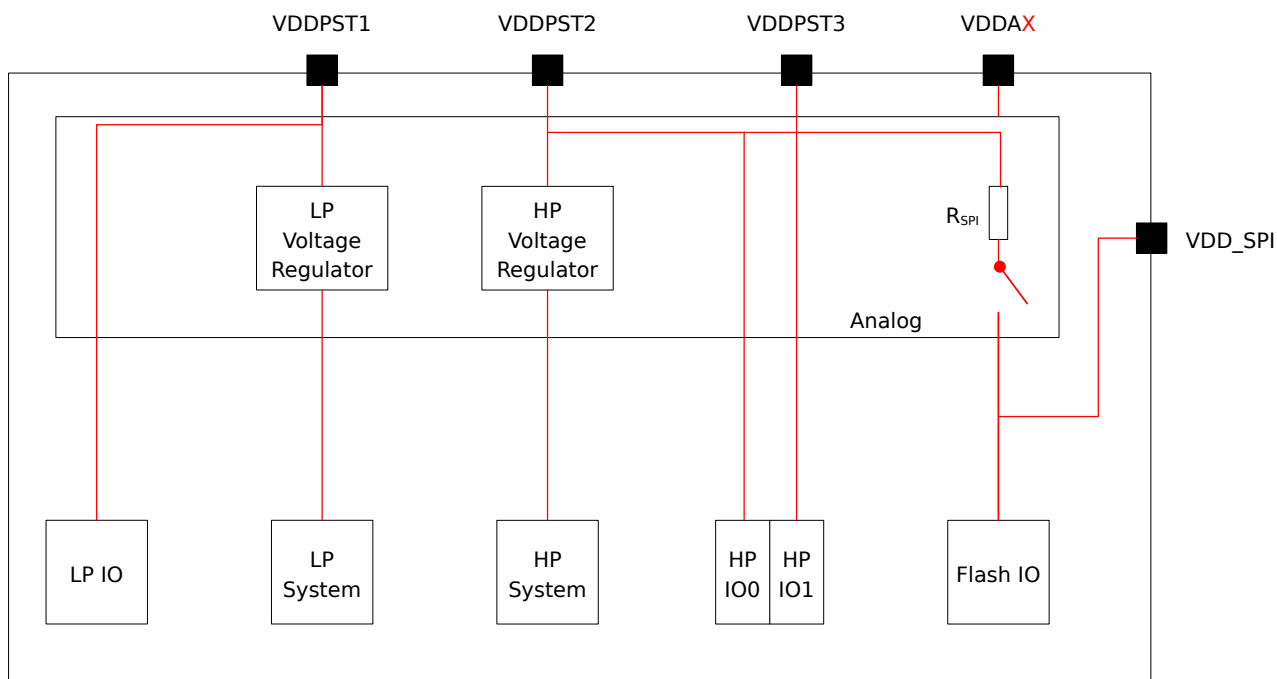
Figure 2-4. ESP32-C5 Power Scheme
