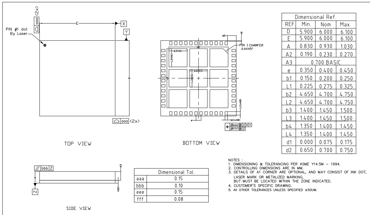
Figure 7-2. LGA48 (6 x 6 mm) Package
