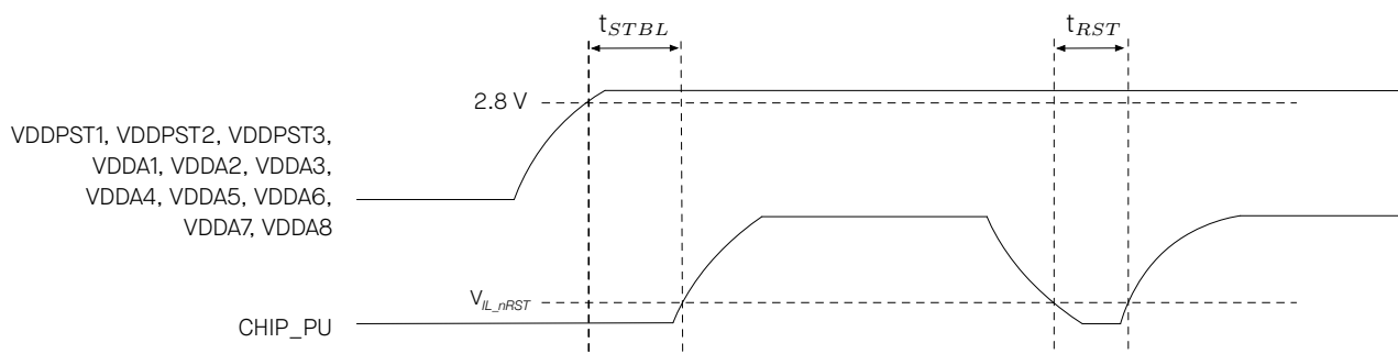
Figure 2-5. Visualization of Timing Parameters for Power-up and Reset
