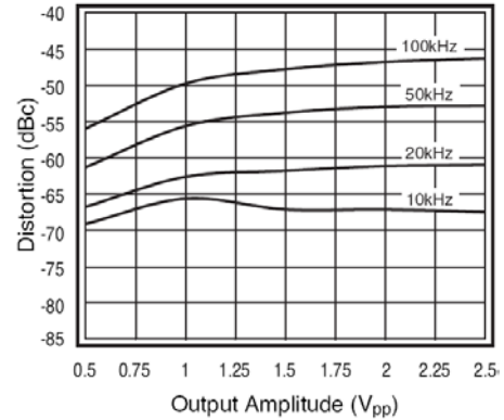
Figure 14. 2nd Harmonic Distortion vs. V_O
