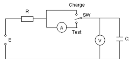
Measurement circuit 测试电路
