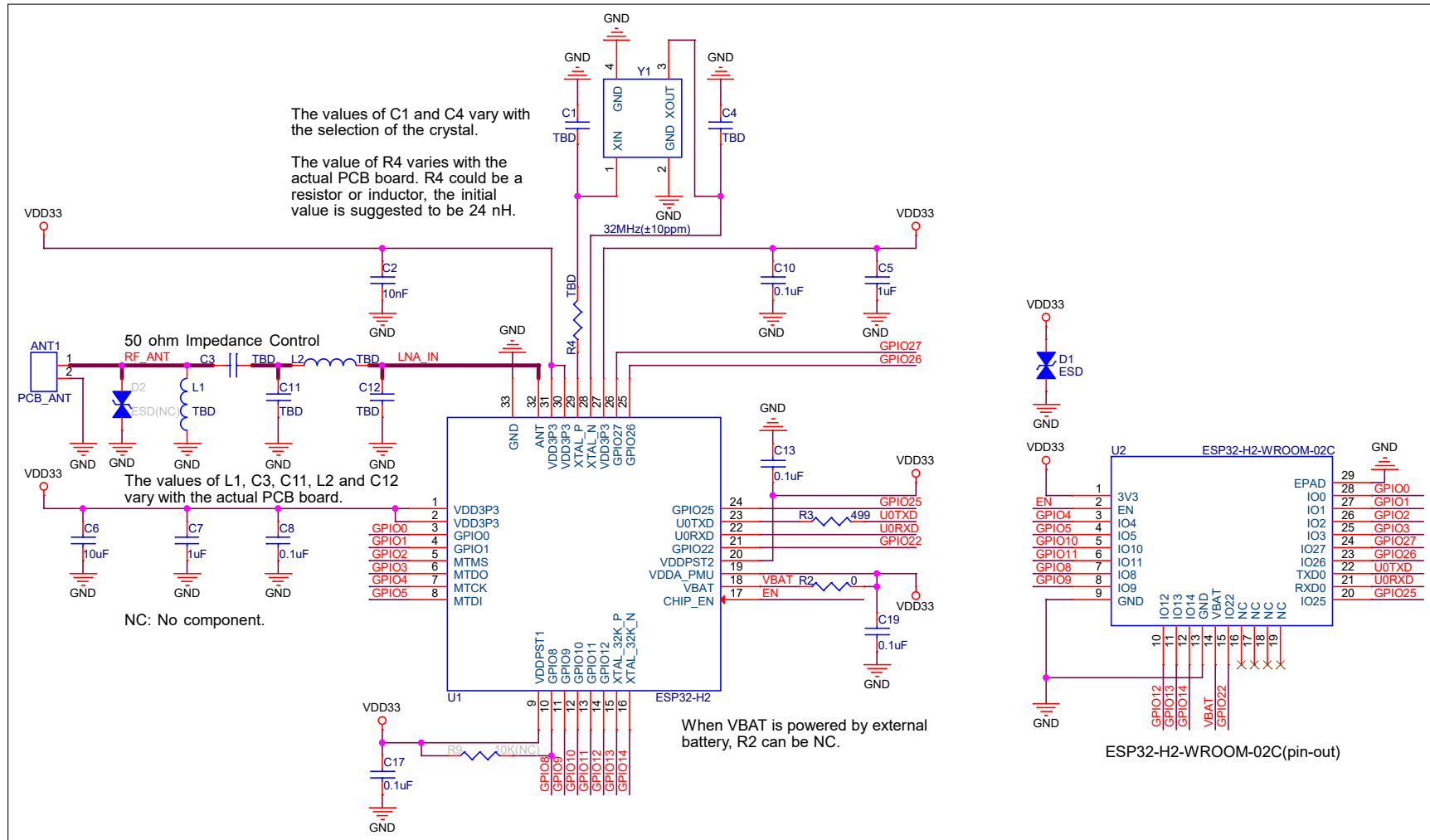
Figure 4: Schematics
