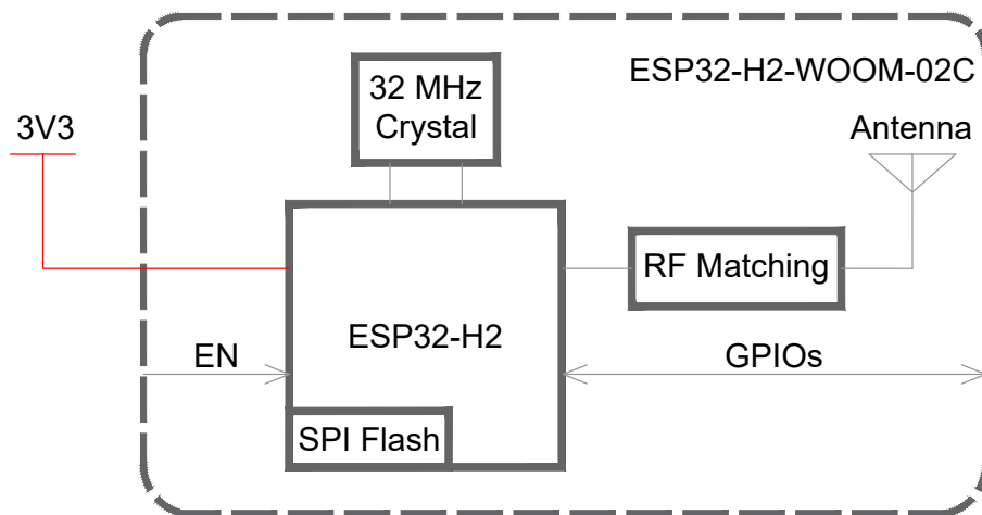
Figure 1: Block Diagram
