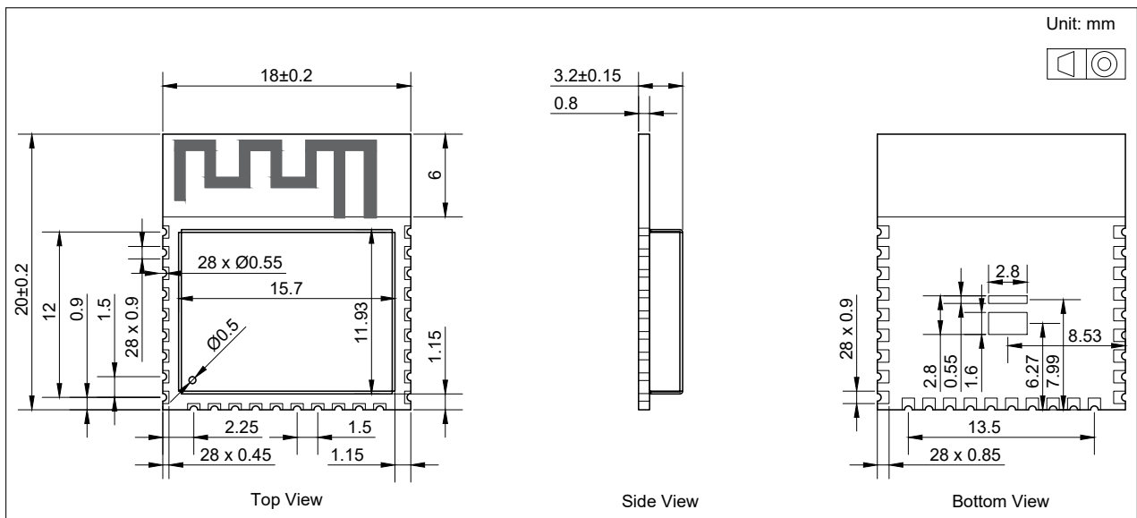
Figure 6: Physical Dimensions
