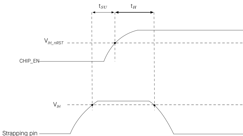
Figure 3: Visualization of Timing Parameters for the Strapping Pins
