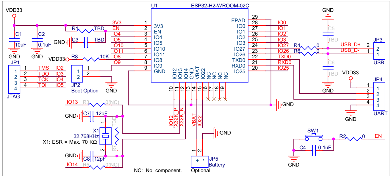
Figure 5: Peripheral Schematics
