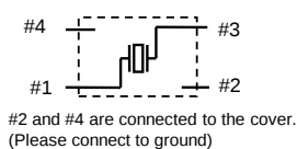
Internal connection (TOP VIEW)
