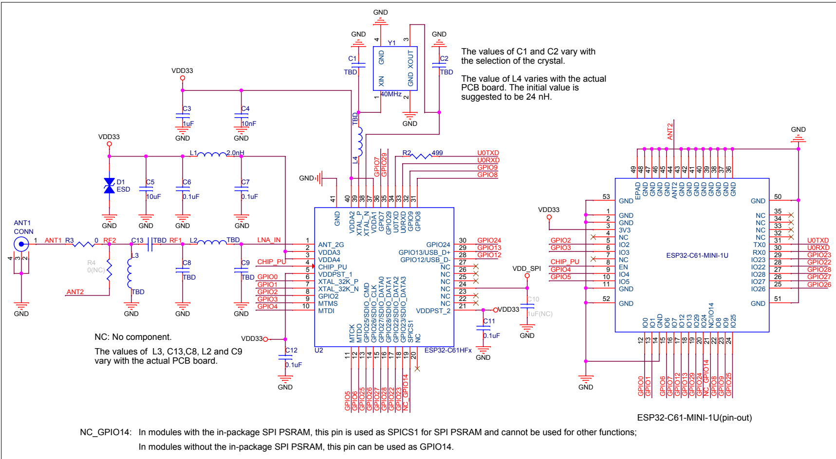
Figure 8: ESP32-C61-MINI-1U Schematics
