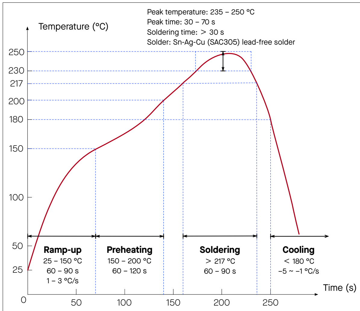
Figure 16: Reflow Profile
