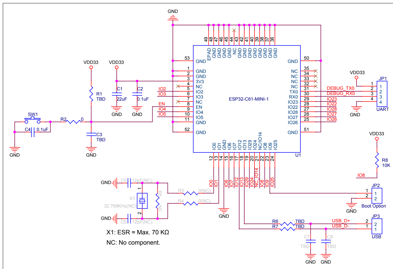
Figure 9: ESP32-C61-MINI-1 Peripheral Schematics
