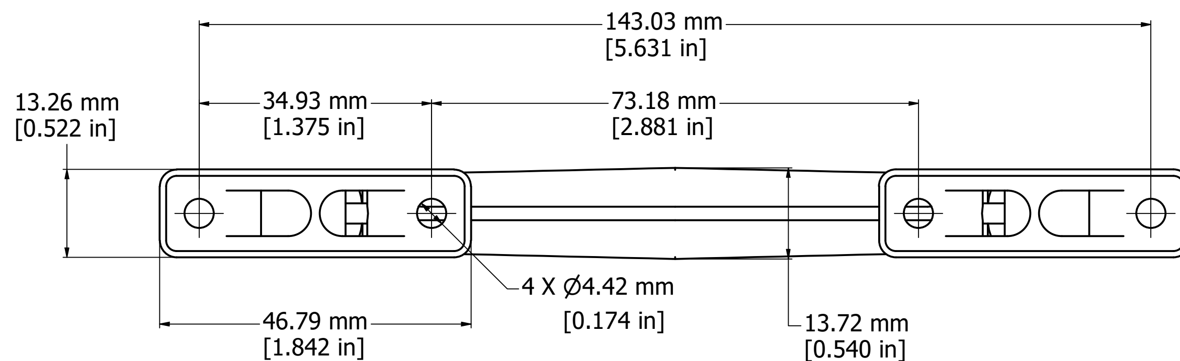
BOTTOM VIEW
