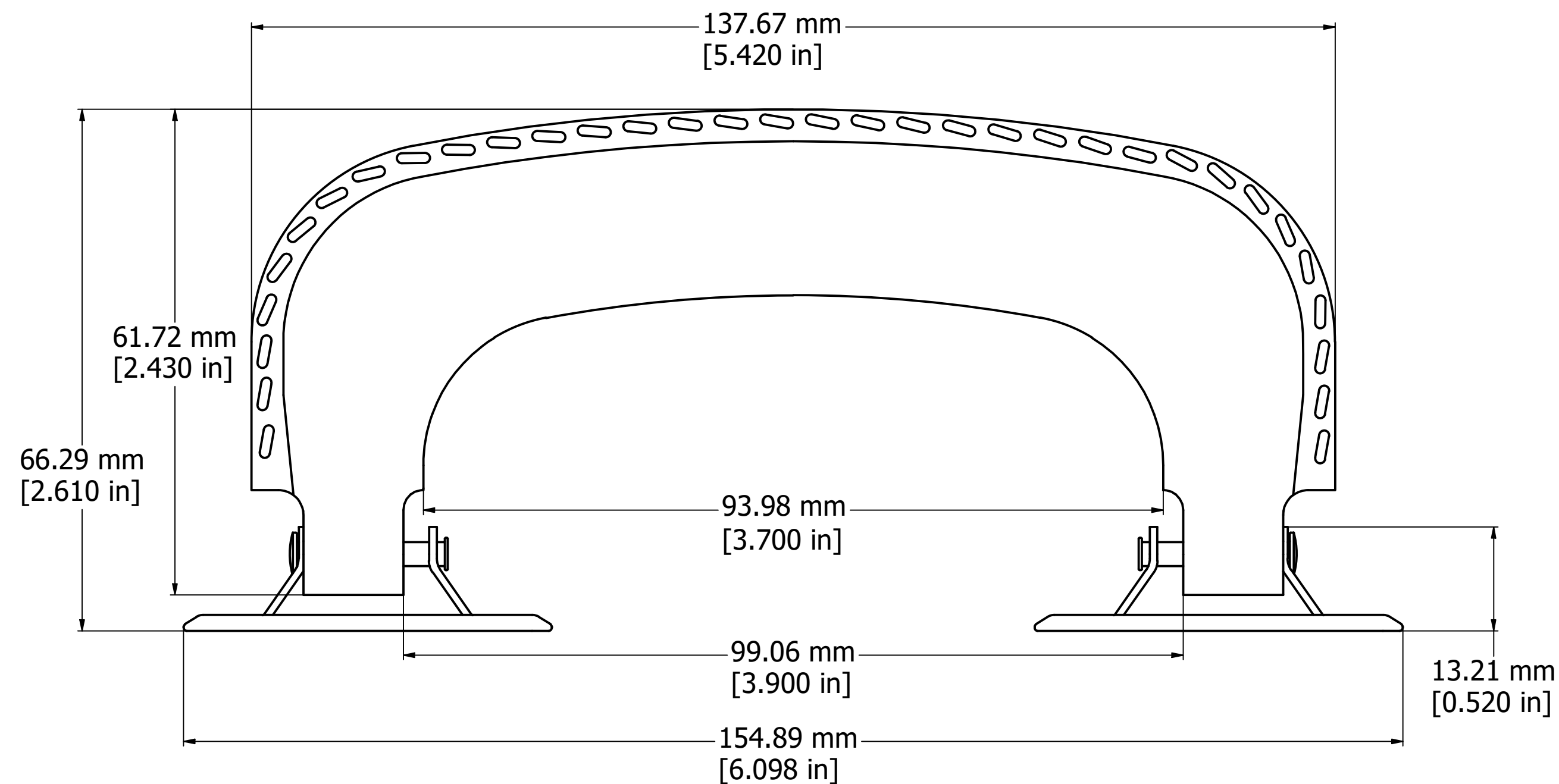
FRONT VIEW
