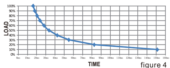
DDR-480C-48
