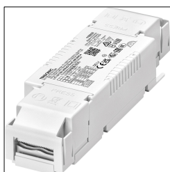
LED-Treiber LC 10/150-250/42 flexC SR SNC4 87501086
